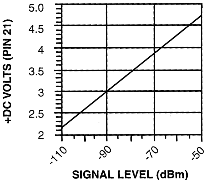
图9 RSSI vs.Vdc(Typical)
